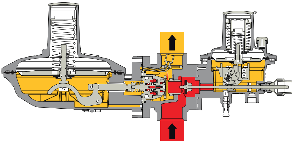
Dival Regulator With LA Slam-Shut
